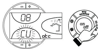
fig. 11 - Compensation curve
