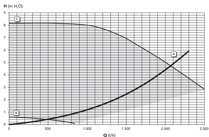
fig. 27 - Circulating pump head / pressure losses
