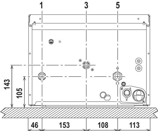
fig. 12 - Raccordements hydrauliques
