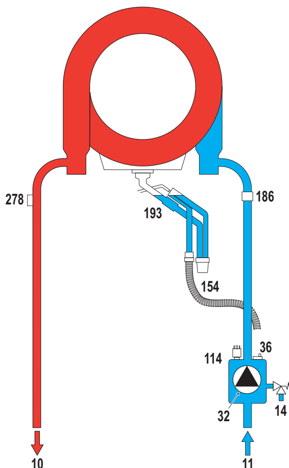
fig. 28 - Hydraulic circuit
