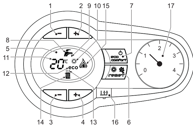
fig. 1 - Control panel
